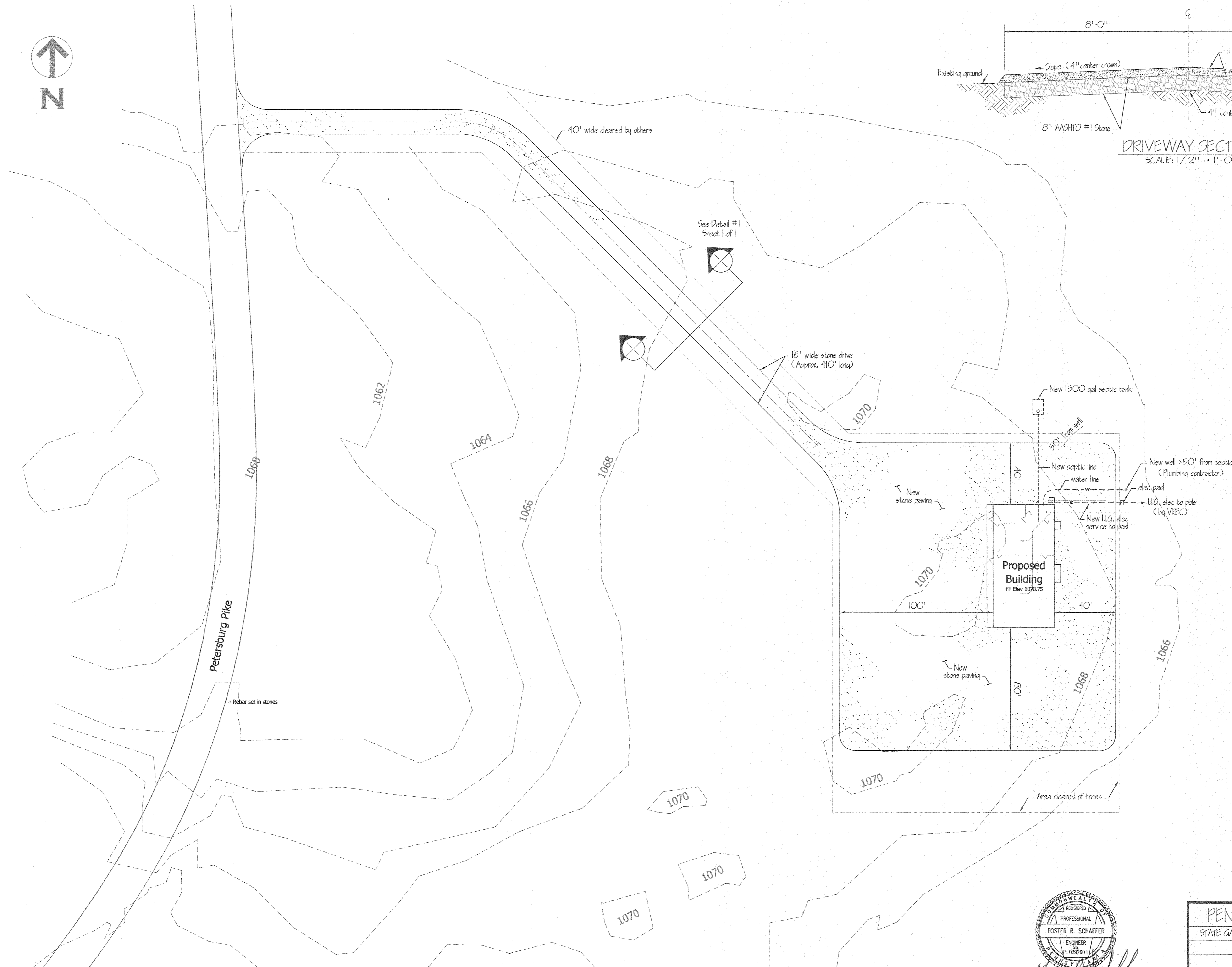
SITE PLAN SCALE: 1" = 30'
